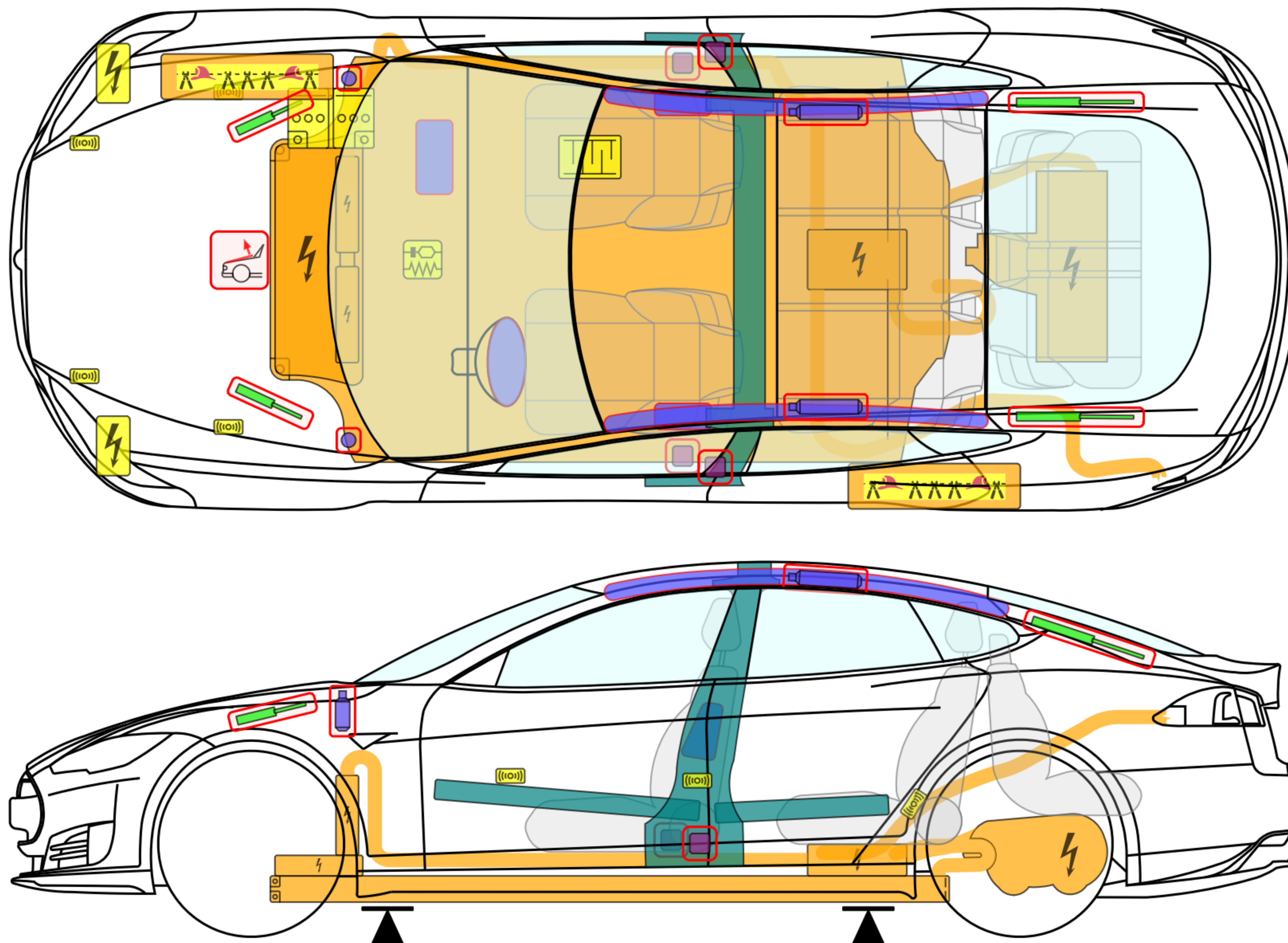
Tesla Model S
