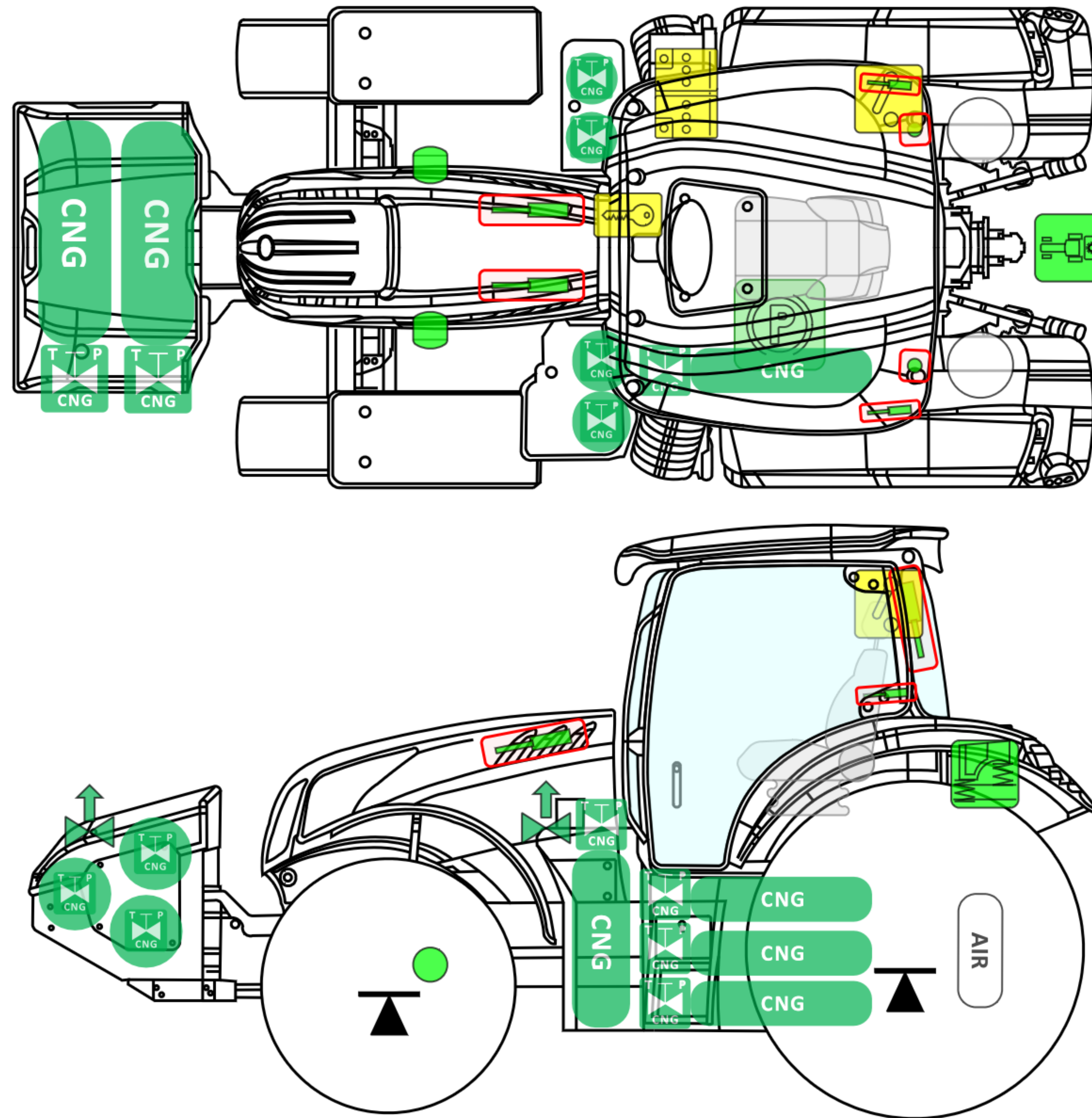
New Holland T6
