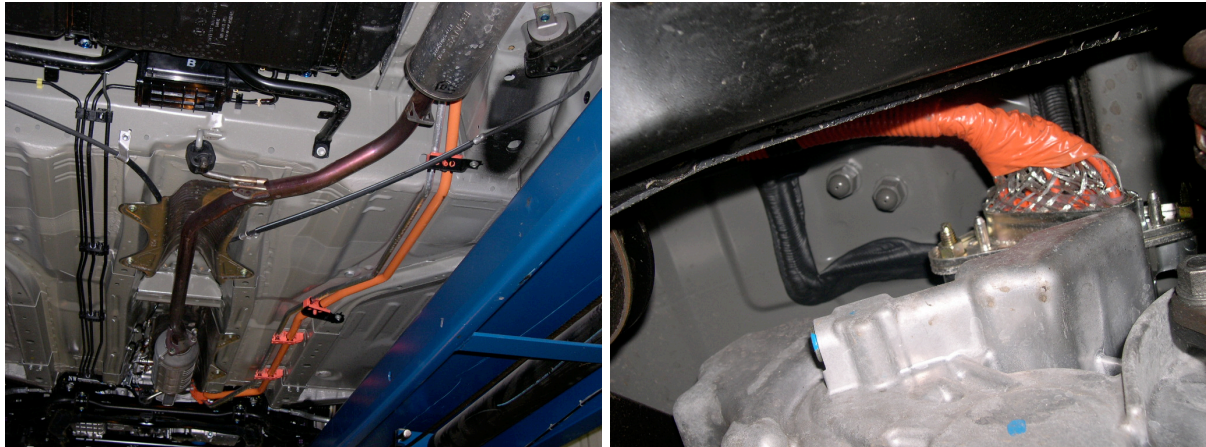
Figure 14: High voltage power cables under the floor pan of Hybrid vehicles (Honda Civic IMA, Lexus RX 400h). In the right photo the wire braid that is used for insulation monitoring is visible.
