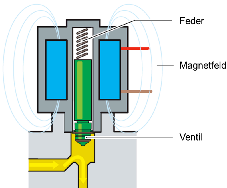
Figure 3: Operating mode of an electromagnetic shut-off valve (courtesy of Volkswagen AG)
