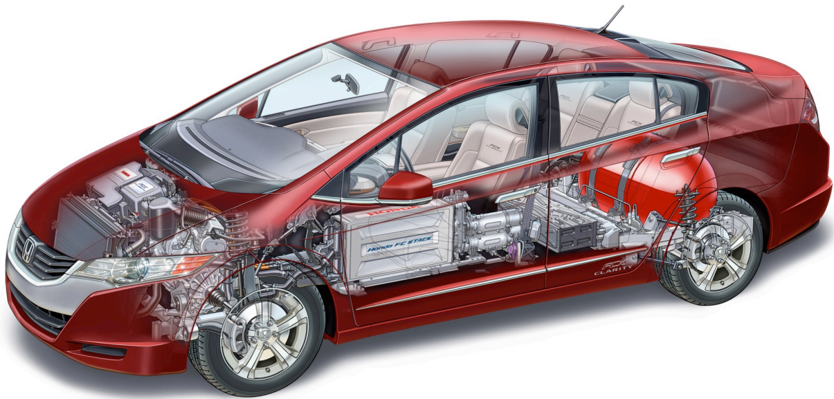
Figure 17: Honda FCX Clarity test vehicle. In this vehicle the hydrogen is stored under pressure (345 bar) and feed a fuel cell. The fuel cell creates electricity to power an electric motor. A high voltage battery is also present (courtesy of Honda).
