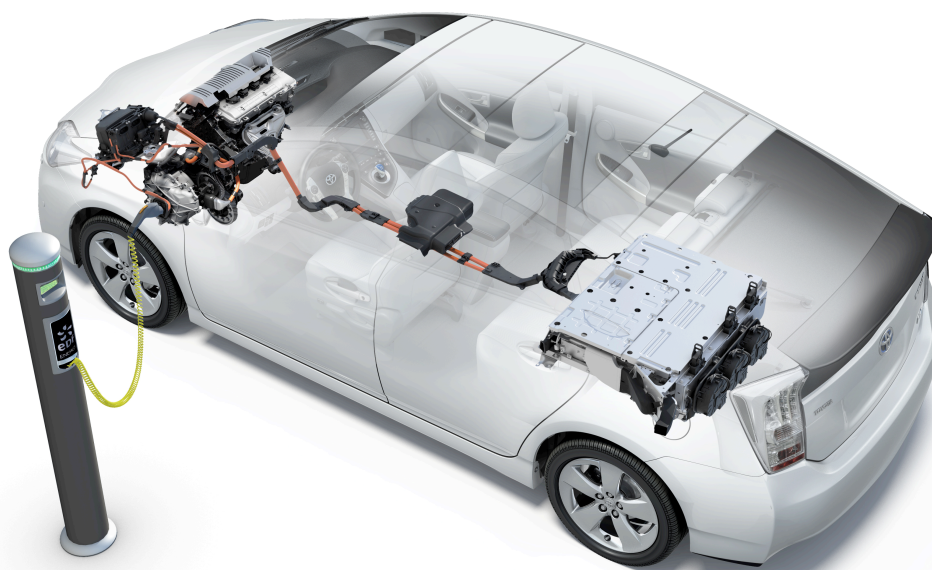
Figure 10: Toyota Prius PHV, Plug-In electric hybrid (courtesy of Toyota)
